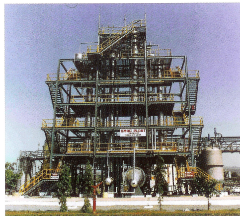
5,000 MTPY Dimethyl Acetamide Plant - India
