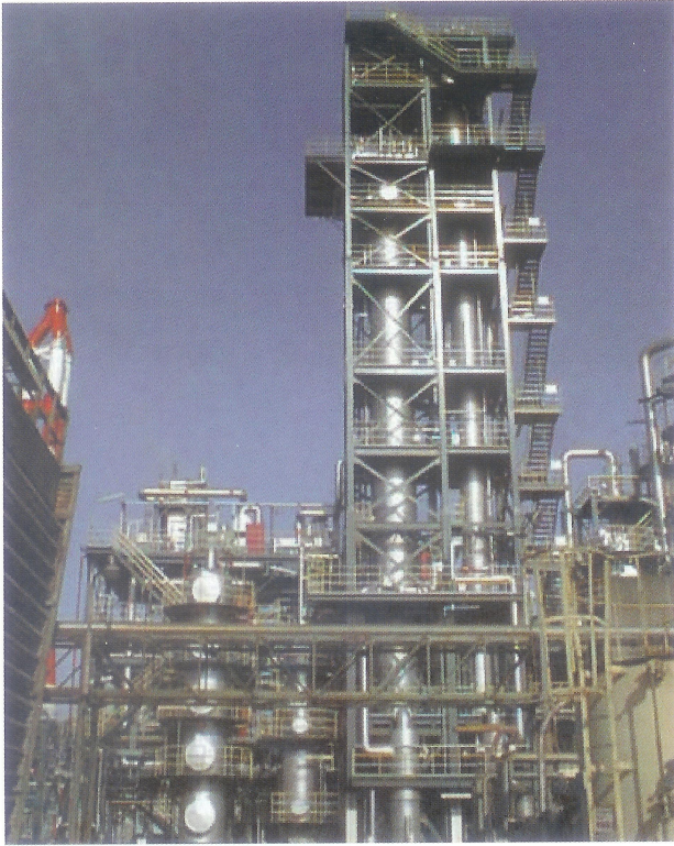
Methylamine Plant – Japan
